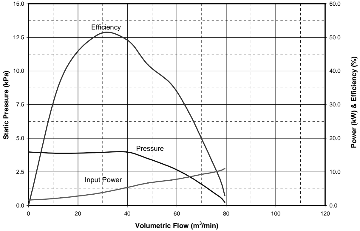
3450 RPM Forward Curve 6" Outlet Fan
