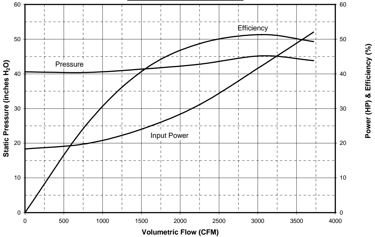
4500 RPM Forward Curve 8" Outlet Fan
