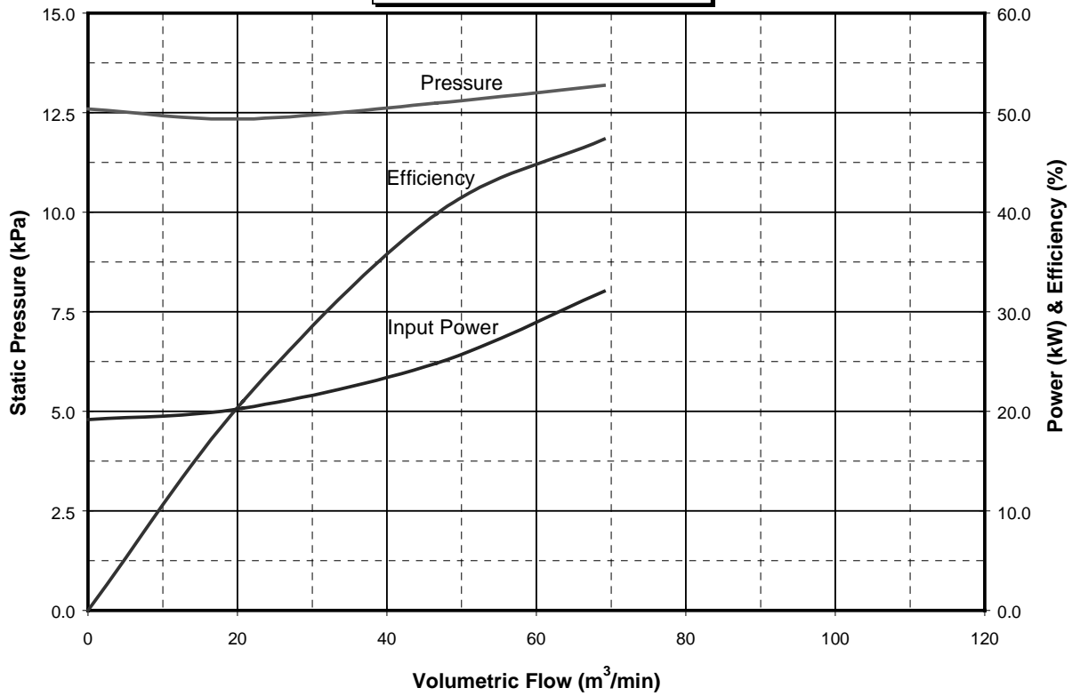
5000 RPM Forward Curve 8" Outlet Fan
