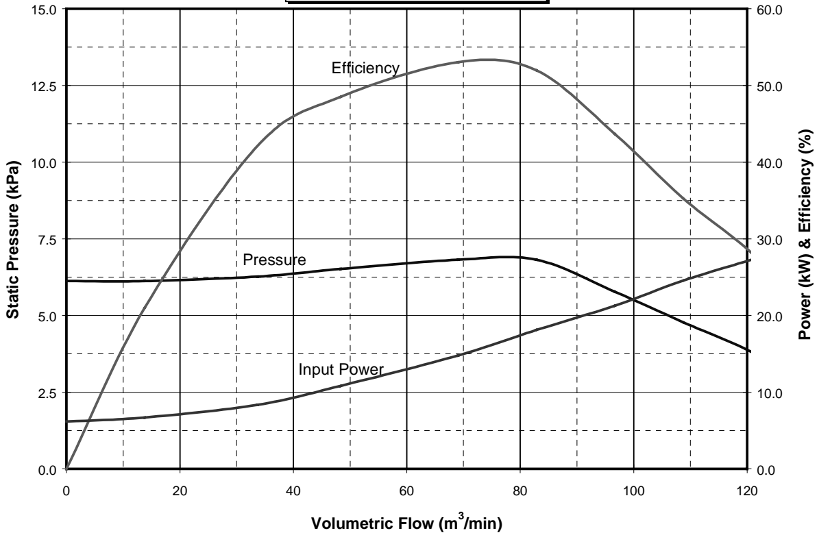
3450 RPM Forward Curve 8" Outlet Fan
