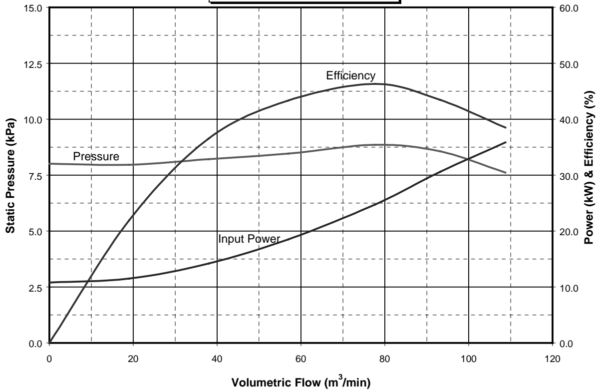
4000 RPM Forward Curve 8" Outlet Fan
